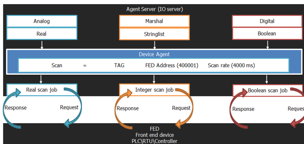
Figure 2 - Scanning subsystem - Solicited/Polled Driver Architecture
