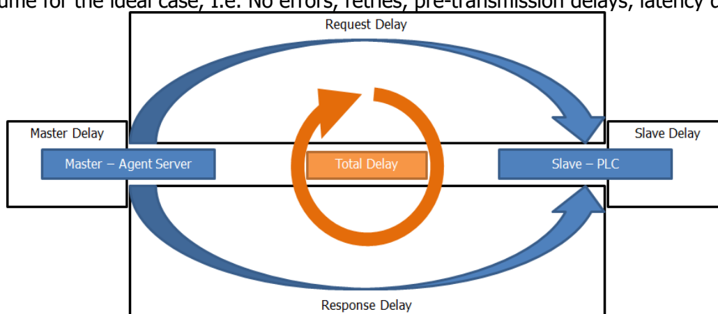
Figure 3 - Scanning transaction time
